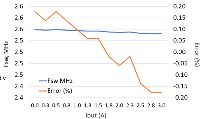
Switching Frequency Accuracy vs Iout ( V_{OUT} = 1.136V )
