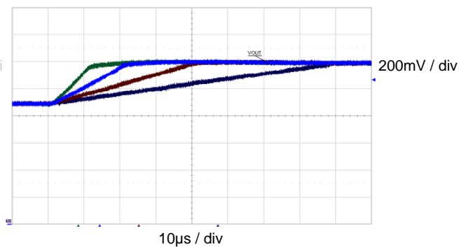
DVS Positive Ramp-Up Rates ( V_{OUT} = 0.9-1.2V )
