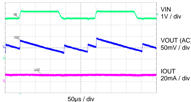
Line Transient Response (V OUT = 1.136V, Mode = Auto)
