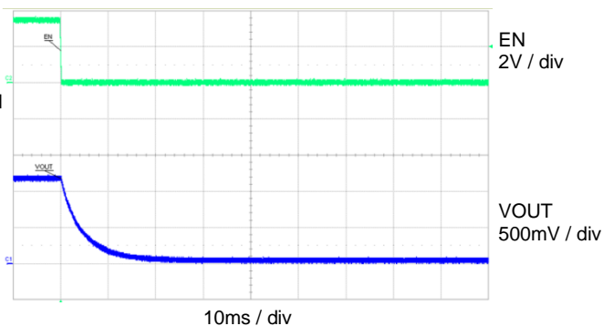
Buck Shutdown ( V_{OUT} = 1.136V , Active Discharge Enabled)
