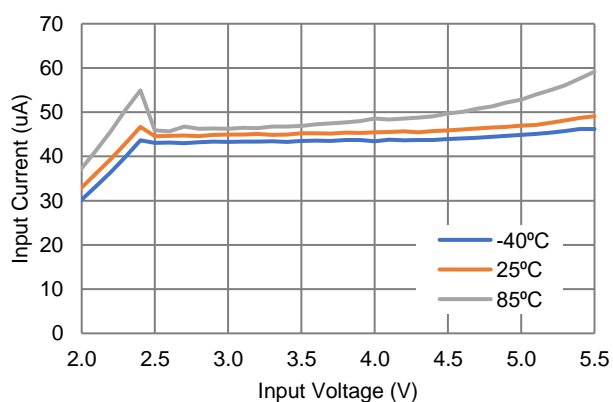
Supply Current vs. V_{IN} ( V_{OUT} = 1.136V , No Load, Mode = Auto)
