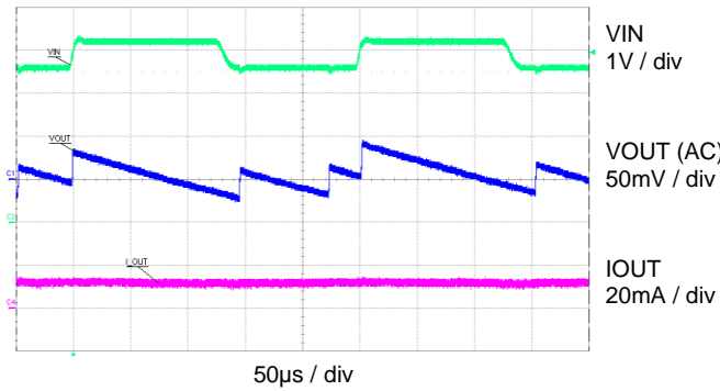
Line Transient Response ( V_{OUT} = 1.136V , Mode = Auto)
