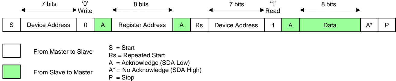
Figure 4. I 2 C Read Cycle
