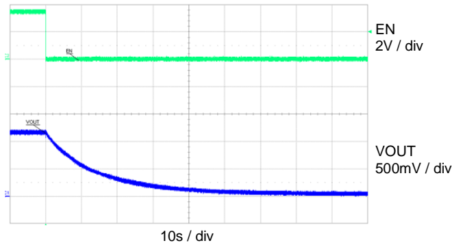
Buck Shutdown ( V_{OUT} = 1.136V , Active Discharge Disabled)
